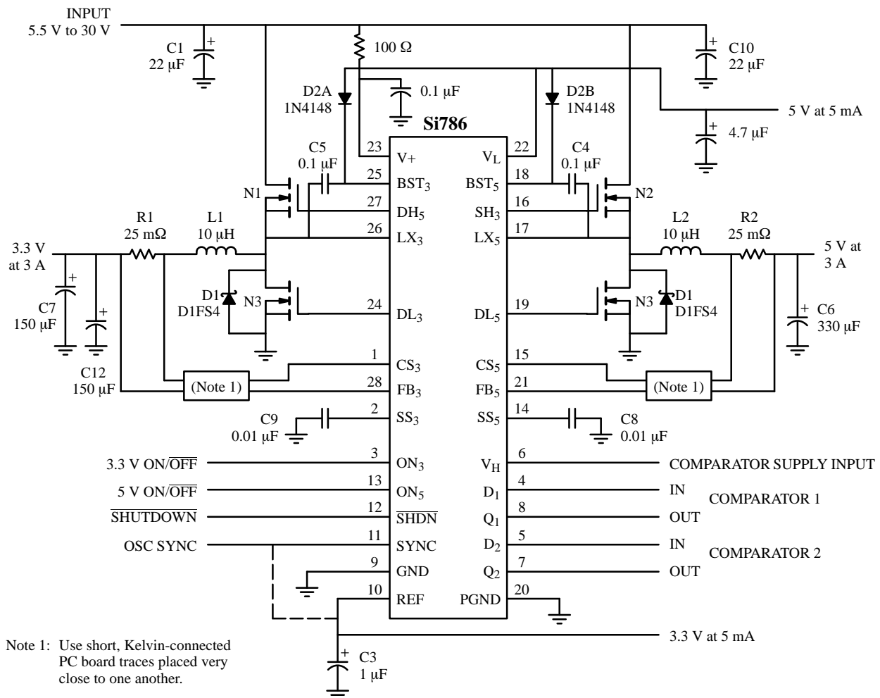
Figure 1. Si786 Application Circuit
