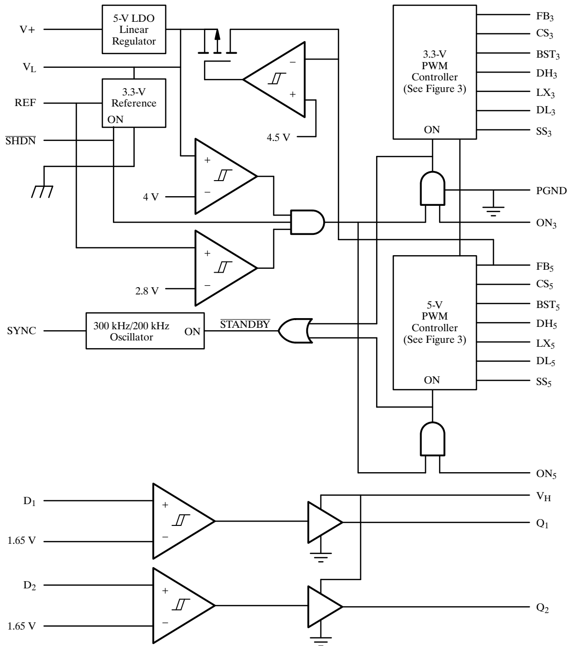
Figure 2. Si786 Block Diagram
